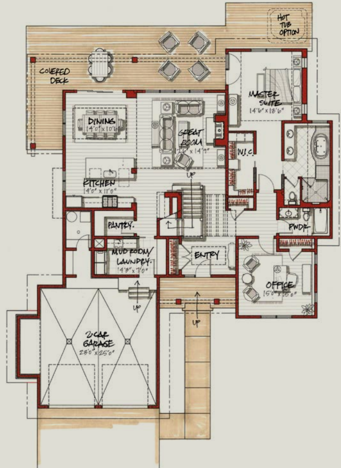
MAIN LEVEL FINISHED: 2064 SQ. FT.
