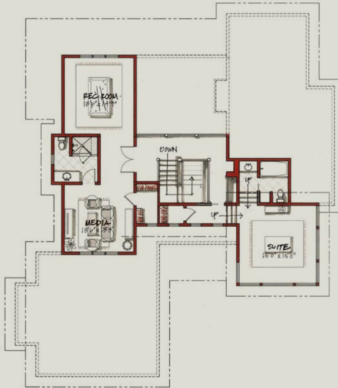
UPPER LEVEL FINISHED: 1265 SQ. FT.
